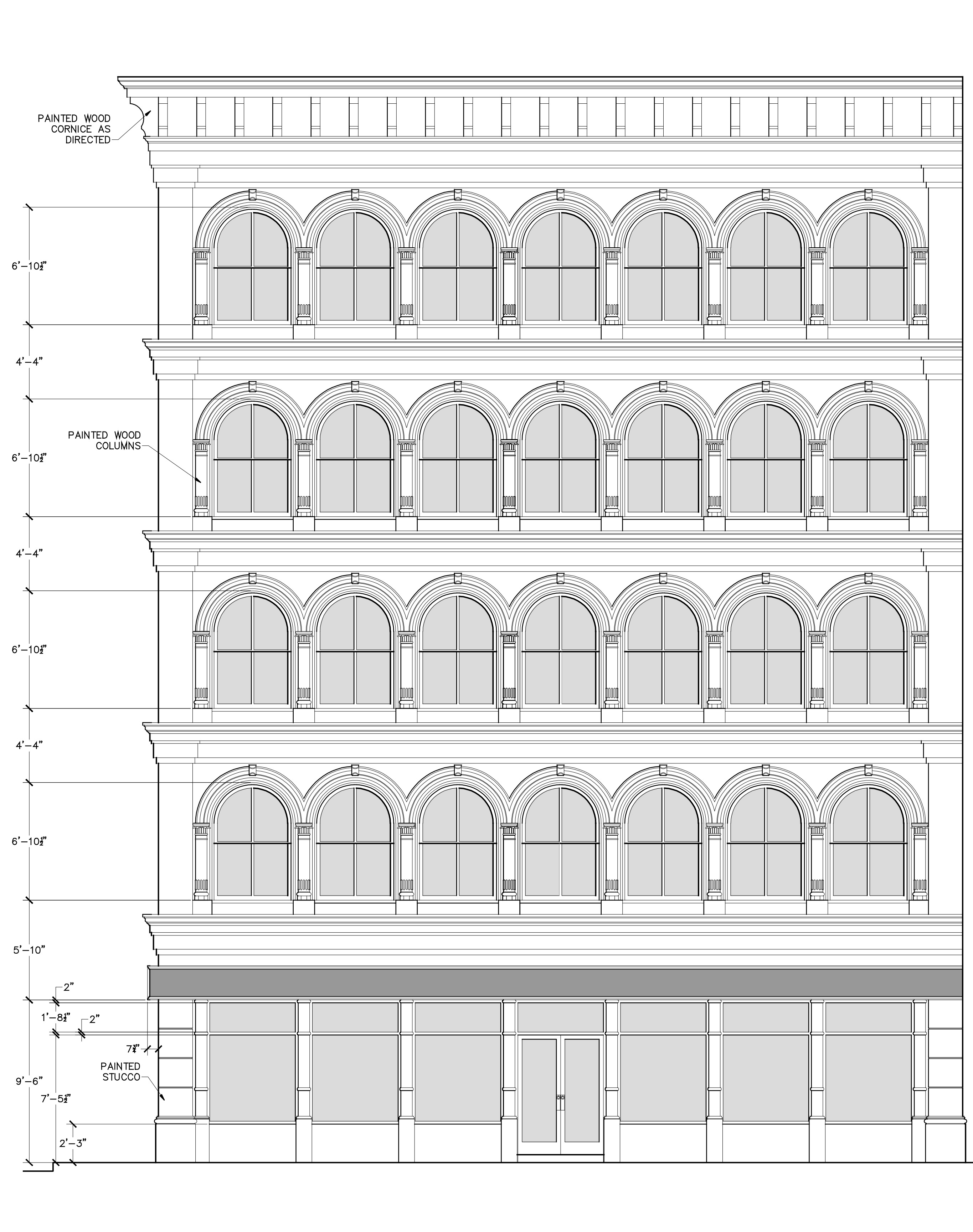
ELEVATION BUILDING #7 B SCALE 1/4" = 1'-0"
