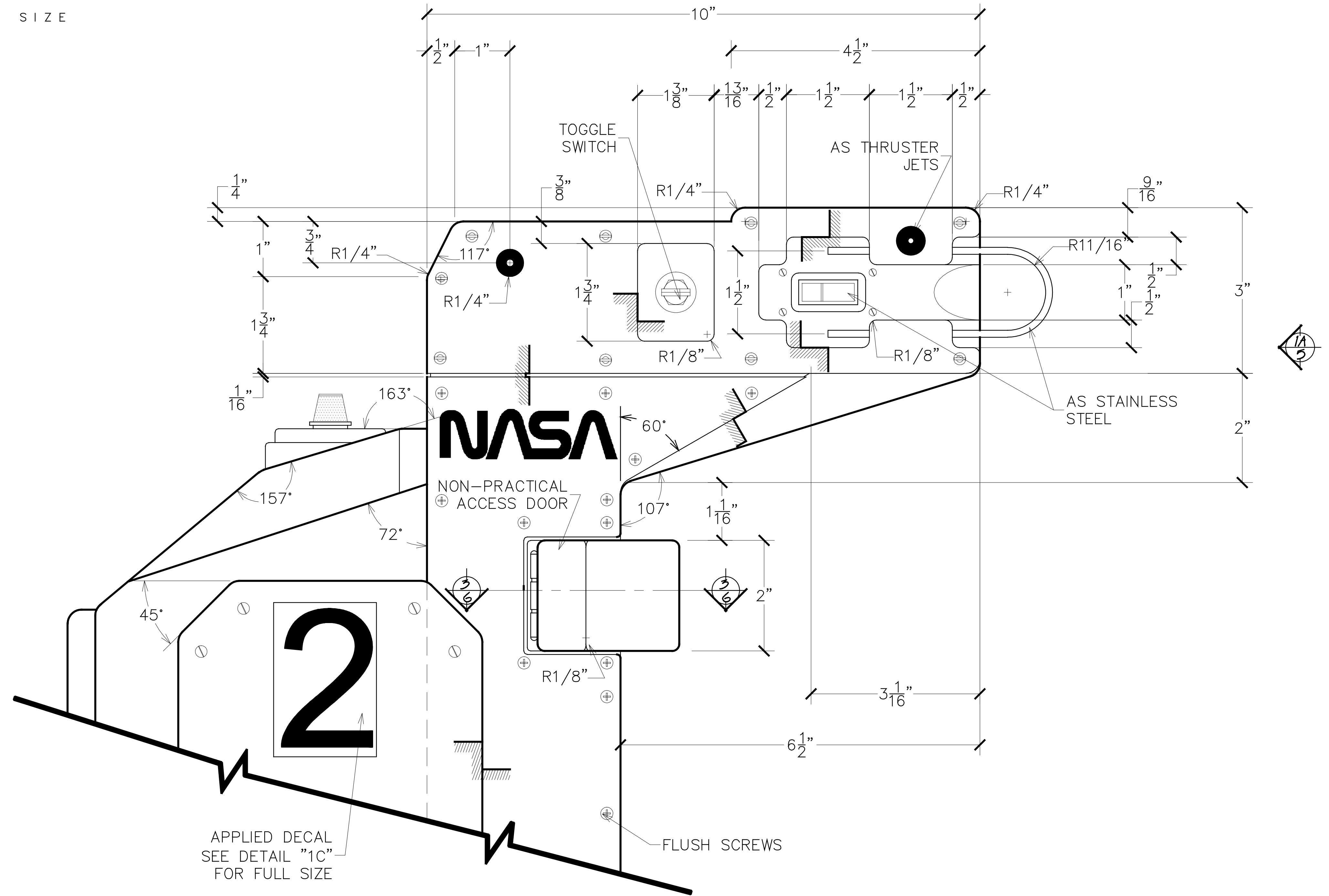
DETAIL (1B) ELEVATION SCALE FULL SIZE
